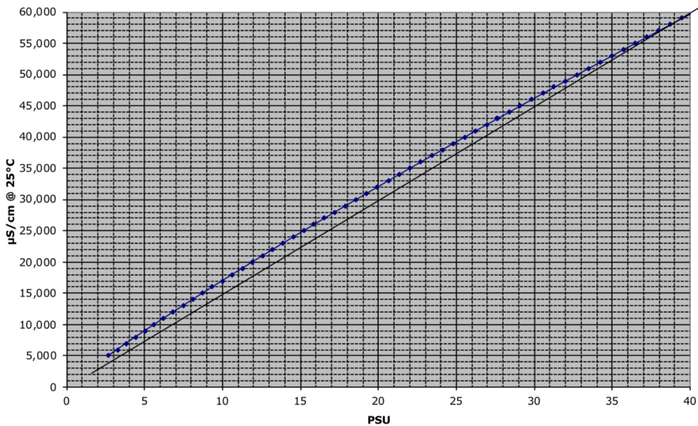
µS/cm @ 25°C vs PSU
