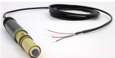
AB 8XX0 Twist Lock Quick Disconnect Inline Silver Halide Series Ion Selective ISE sensor with no preamplifier
