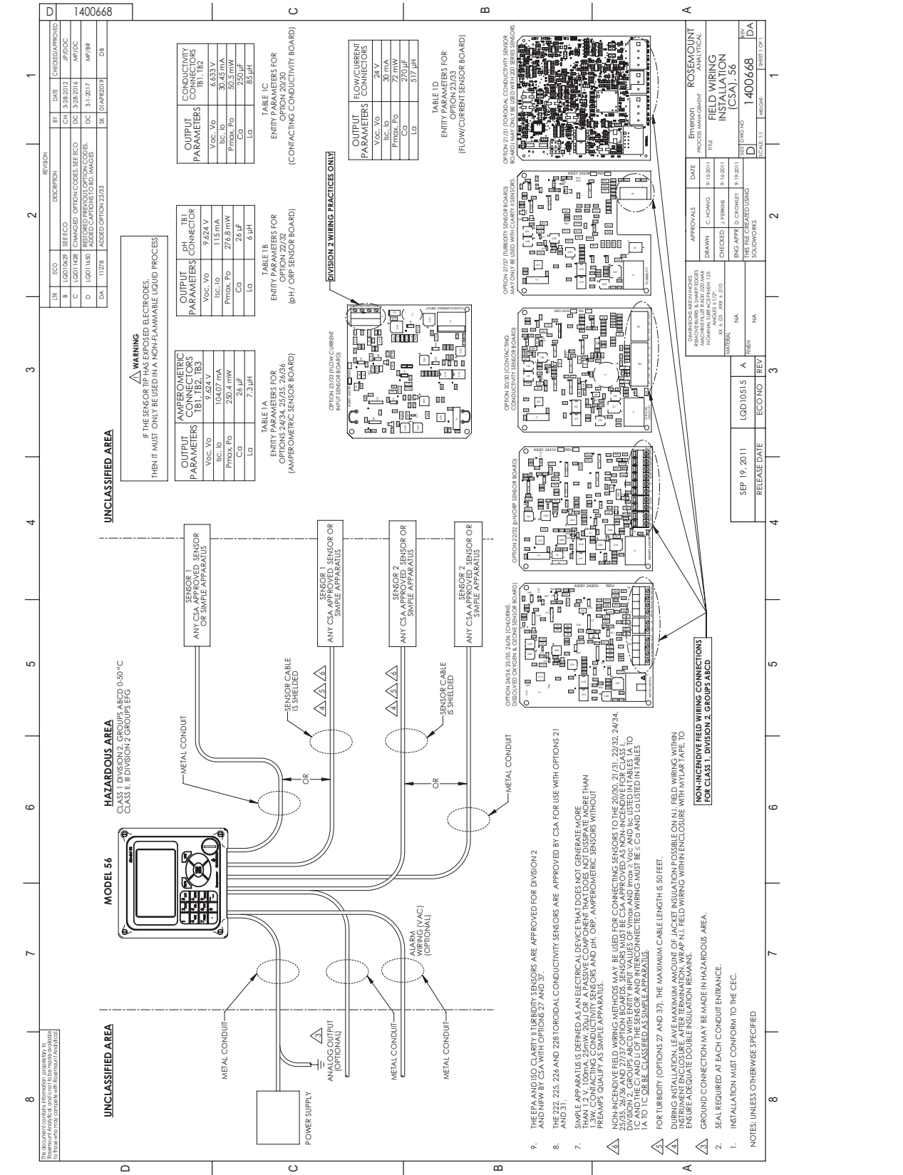
Fig. 2-4 CSA Non-incendive field wiring installation
